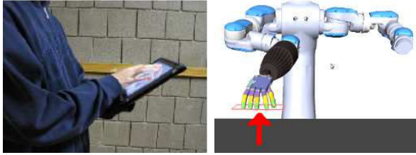
Fig. 6. Device Tilting: The operator tilts the device and holds it beyond a predefined angle to “scroll” the hand upwards.
