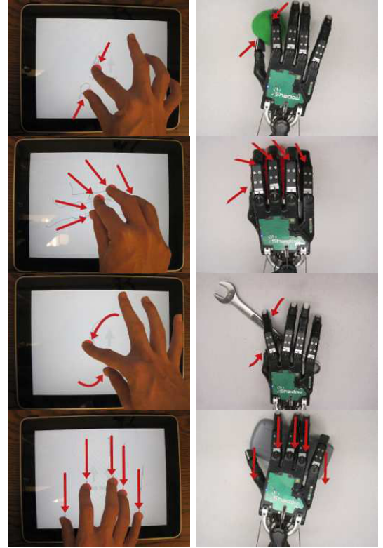
Fig. 1. Multi-touch telemanipulation: From top to bottom, two-fingered pinching, five-fingered power grasp, two-point rotation and sliding
