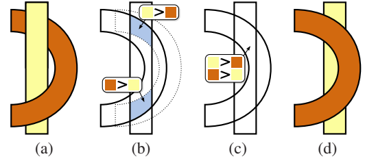
Figure 11: Starting with configuration (a) the user moves the crescent to the left. The votes, (b), are inconsistent in the central region, (c). Picking a consistent subset will result in popping (one possibility shown in (d)). Depending on a user toggle, we can instead roll back the edit.
