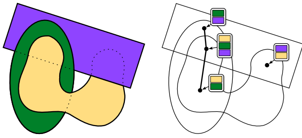
Figure 5: Left, an example figure containing three objects. Dotted lines indicate occluded contours. Right, the corresponding regions of overlap and list-graph. Lists containing one or fewer elements are not shown.
