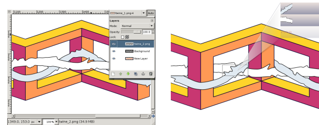
Figure 2: Left: A standard paint program (GIMP pictured) provides only a global ordering of layers. Right: Our local layering prototype allows a different ordering in each region of overlap. Here the local layering dialog is being used to control the overlap of the white and gray ropes at one of their crossing points.
