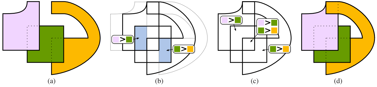
Figure 9: Maintaining a temporally coherent stacking. (a) The original stacking. (b) The updated layer positions, with local votes cast in the image-space overlap between the old stacking regions (dotted) and the new (solid). (c) After vote propagation. (d) Final stacking; all votes satisfied. The overlap at the top was not constrained, so was chosen based on a given tie-breaking order (here prioritizing the orange crescent).
