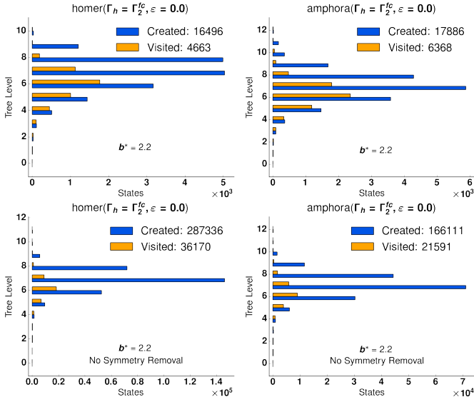
Figure 6. Created and visited states for A* SEARCH with and without symmetry removal. Most states are considered on the middle levels in the search tree. Effective branching factors are shown as b^* . Note that the total number of possible states is approximately: \sum_{i=0}^{\log_2} |C| (b^m)^i \approx 1, 227, 133, 513 .
