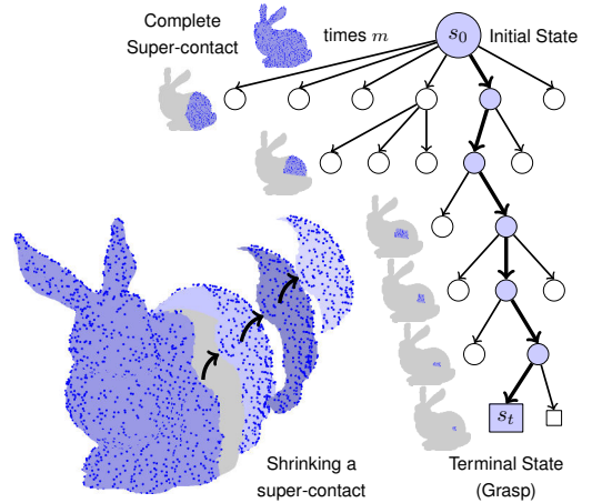
Figure 1. Our approach is based on reducing optimal grasping to finding a minimal cost path. Starting with complete super-contacts that cover the whole object, we step-by-step remove contacts until we reach m -contact grasps. Each state is a combination of m super-contacts and each arc shrinks the included super-contacts. The minimal cost path ends at the optimal grasp.
