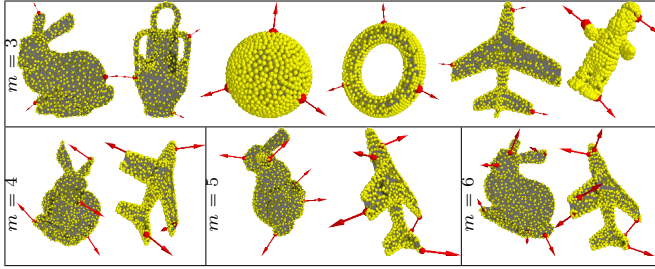
Figure 3. Optimal grasps with m = 3 contacts found by our approach using A^* SEARCH shown by arrows for the objects bunny , amphora , sphere , donut , plane , and homer and with m = 4, 5 and 6 for bunny and plane . The contact set C is indicated in yellow. The results obtained are identical to ES.
