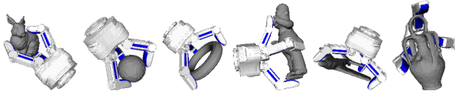
Figure 10. Constraints on grasps: Optimal kinematically feasible grasps by Schunk-SDH hand for 3 fingertip contacts.
