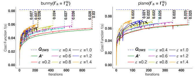
Figure 8. Combined cost plotted against iterations WA* SEARCH using \Gamma_h = \Gamma_4^{fc} . Larger inflation factors \varepsilon lead to less computation. Dashed lines show solution qualities.
