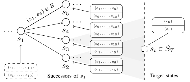
Figure 2. A reducing and preserving successor function \Gamma defines a search graph based on super-contacts s_i . The grasp set \mathbf{G}(s_1) = \{c_1, \dots, c_{10}\}^2 is represented by all states s_i \in \Gamma(s_1) together where the grasp sets of successor states of s_1 are strictly smaller than \mathbf{G}(s_1) . Since the grasp (c_6, c_1) is represented by two successors, G is not necessarily a tree. However, G can be constructed as a tree if the partitions do not overlap. For this figure m = 2 .
