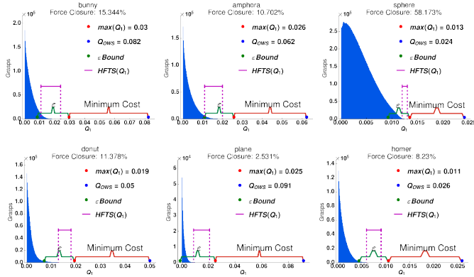
Figure 4. Comparison between ES, HFTS, and our approach for m = 3 . Histograms (blue) show the Q_1 quality distributions for each object. Minimum path cost indicates the quality drop from q(s_0) = Q_{OWS} to the optimal solution g(s_t) . Empirical standard deviation shows large quality variance for HFTS. A^* SEARCH identifies the optimal solution (red) and \epsilon = 0.4 bounds (green) show ranges of bounded sub-optimality results.
