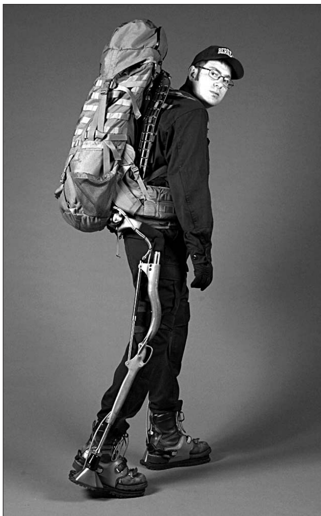
Figure 4. BLEEX exoskeleton. Copyright Berkeley Robotics and Human Engineering Laboratory
