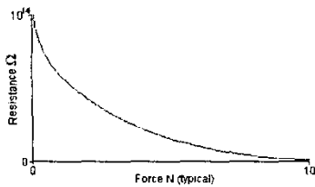
Figure 3. QTC response
