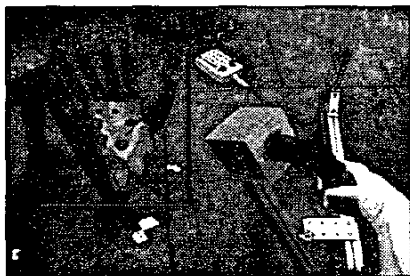
Figure 7. Robonaut gloved hand grasping drill in holster
