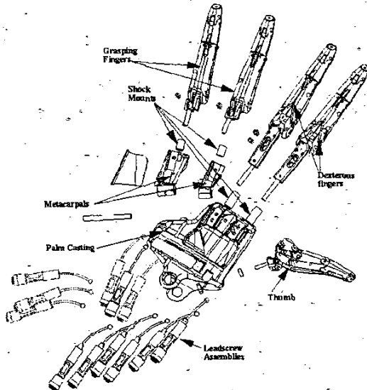
Figure 2. Robonaut hand parts
