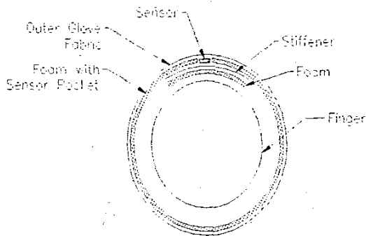
Figure 6. Interlink sensor packaging (cross-section) not-to-scale
