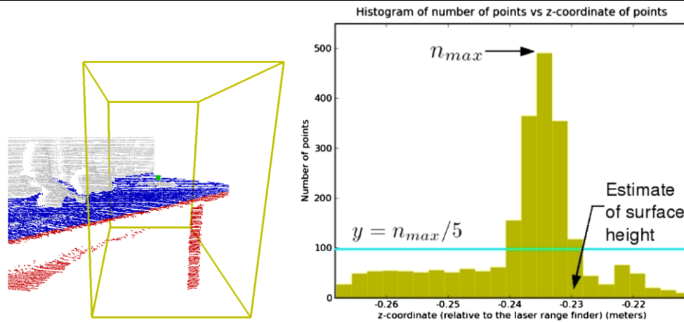
Fig. 6 (Color online) Left : This figure shows the output of the plane detection and segmentation algorithm. The grey , blue and red points are those that are above the surface, part of the surface and below the surface respectively. The yellow lines represent the boundary of the volume of interest around the user-selected location ( green dot ). Right : This histogram is for the part of the point cloud shown on the left that is inside the volume of interest (inside the yellow box ). The X -axis is the
