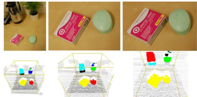
Fig. 15 (Color online) This figure shows the output of the object segmentation algorithm ( bottom row ) as the distance between the two objects is decreased from 6 cm to 2 cm to 1 cm (left to right). When the distance between the objects equals the horizontal resolution of the occupancy grid (1 cm) the segmentation algorithm merges the soap and the medicine box into one object (shown in yellow )
