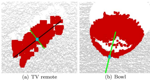
Fig. 10 (Color online) This figure shows the output of the algorithm for selecting the position and orientation for grasping. The robot will try to grasp a TV remote at the centroid with the fingers oriented perpendicular to the direction of maximum variance ( black line ). For the bowl, it will try an overhead grasp at a raised point on the object that is close to the manipulator. In this case, it will orient the fingers along the line joining the grasp position and the centroid of the segmented object. The blue dot and green line indicate the commanded position of the gripper and orientation of the fingers respectively
