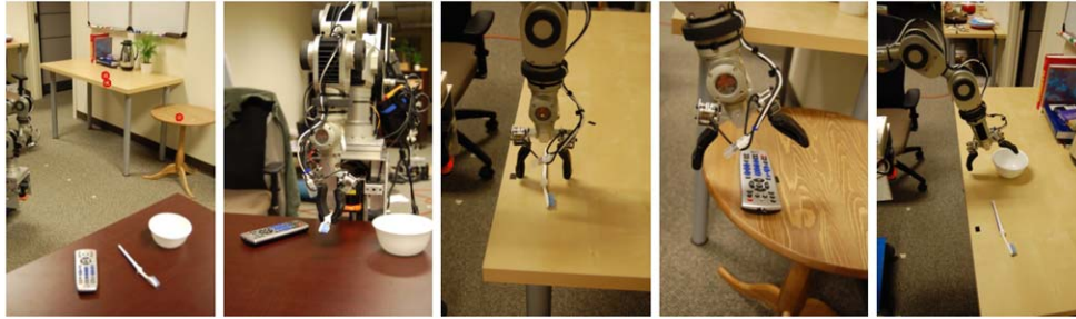
Fig. 14 (Color online) This figure shows the object placement experiment. The first image shows the three objects (TV remote, toothbrush and bowl) and the desired placement points ( red circles ). The second
