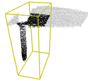
Fig. 11 (Color online) This figure shows the point cloud ( grey and black ) and an approximate volume that the manipulator will sweep out if it executes an overhead grasp ( yellow ). The points within the volume that the manipulator is likely to collide with are shown in black. In this example, the robot detects that an overhead grasp could result in a collision and does not execute the behavior
