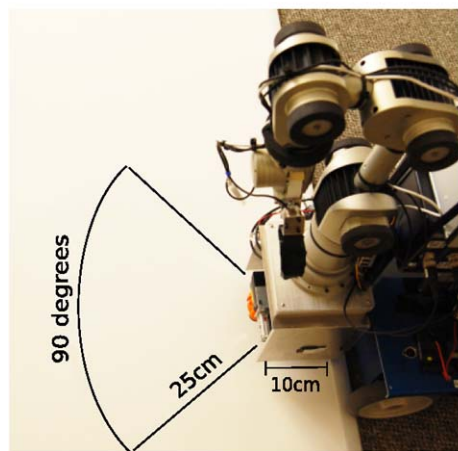
Fig. 8 (Color online) Left : This figure shows the workspace of the overhead grasp behavior. In the radial direction it ranges from 10 cm to 35 cm from the manipulator. The angular limits are imposed by the field of view of the laser range finder which is currently -45^\circ and 45^\circ , due to the design of the carriage. Right : This figure shows how the robot selects the direction to approach a flat surface. The green dot is the user-selected location and the cube defined by the yellow lines
