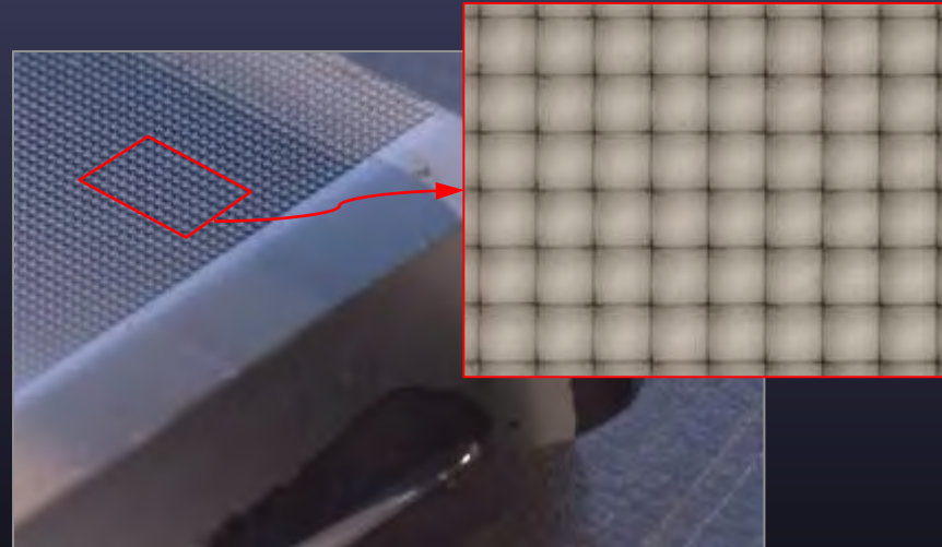
125 \mu square-sided microlenses
